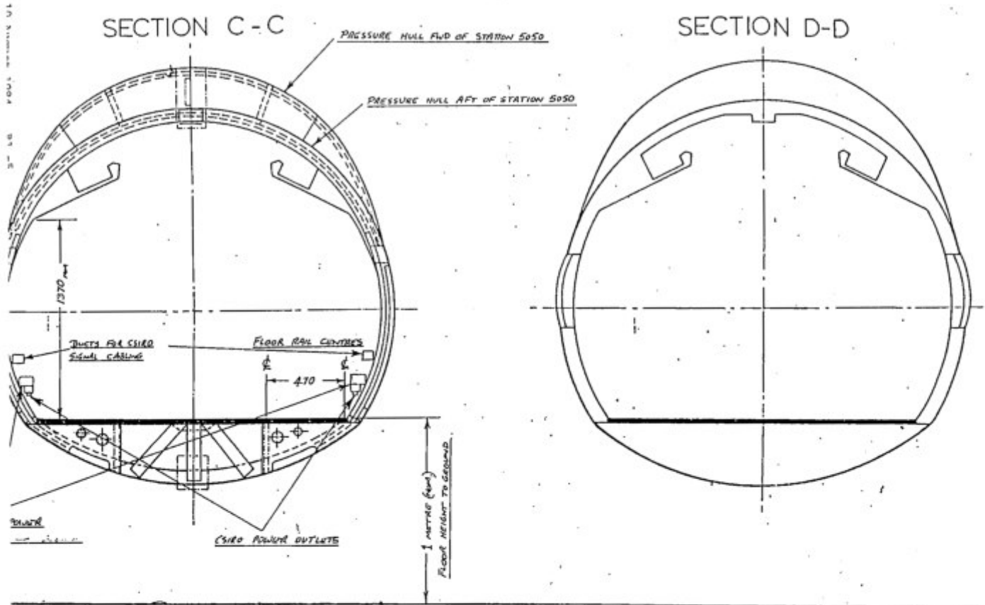
FIG. 4 TYPICAL CABIN CROSS-SECTIONS
